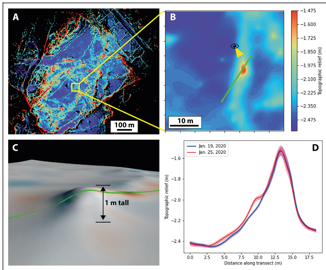
Figure 6. Snow redistribution observed via terrestrial laser scanning (TLS). (A) Complete TLS scan from January 25, 2020, colored by topographic relief; (B) 40 \times 40 m close up of that scan; (C) perspective view from the viewpoint (eyeball and yellow triangle in [B] toward the ridge); and (D) comparison of the topographic relief along the transect line for both scans, with 95% confidence intervals for the surface reconstruction in each profile shown in shading. DOI: https://doi.org/10.1525/elementa.2021.000046.f6
